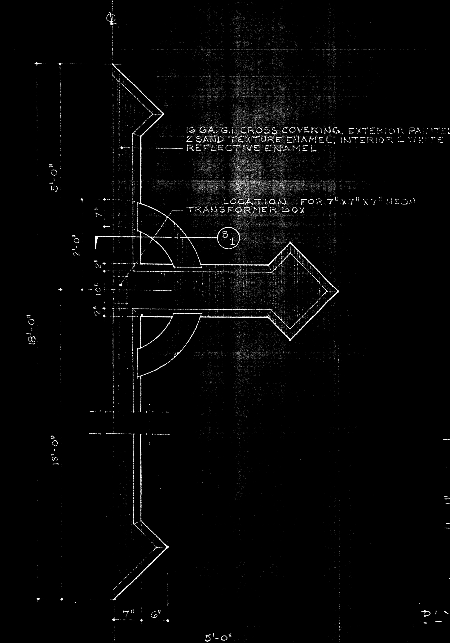
HALF ELEVATION, NORTH WALL CROSS (B)
