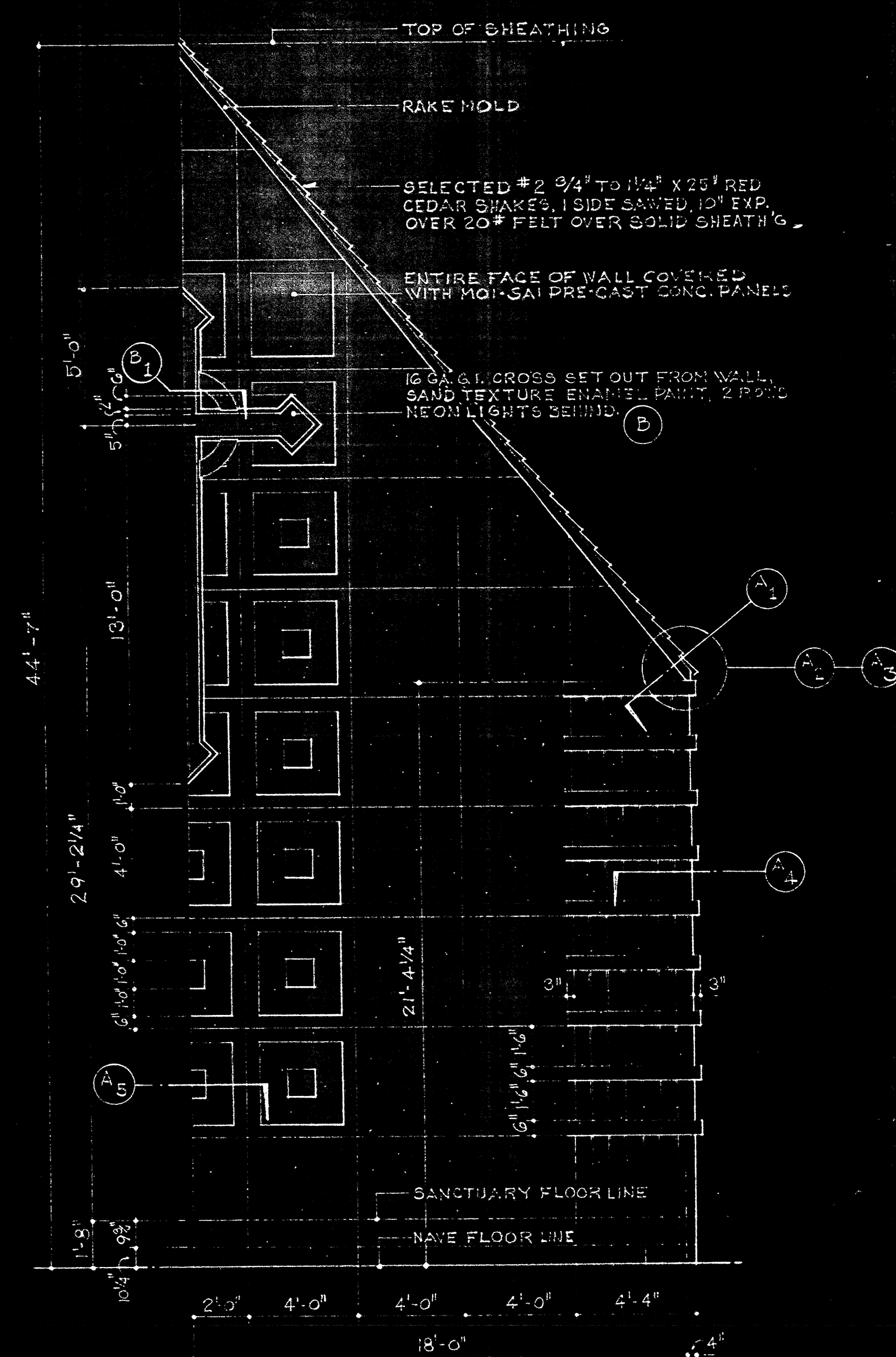
HALF ELEVATION NORTH WALL (A)
