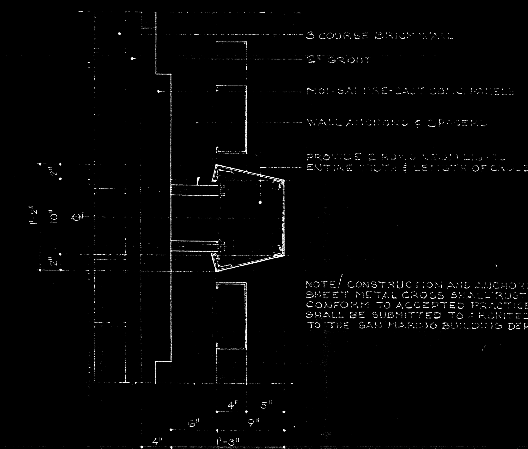
SECTION AT NORTH VALLEY CROSSING
